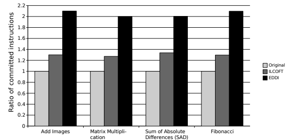
Fig. 4. Committed instructions
