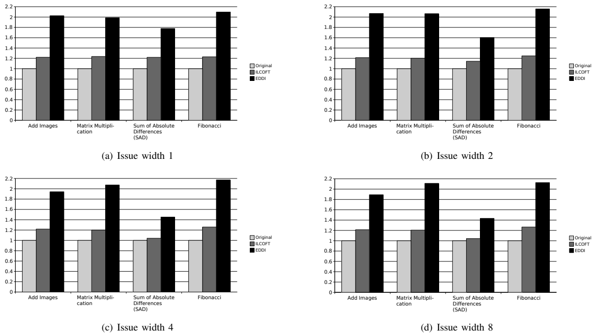
Fig. 5. Energy consumption increase of EDDI and ILCOFT-enabled EDDI over non-redundant kernels, for varying issue widths
