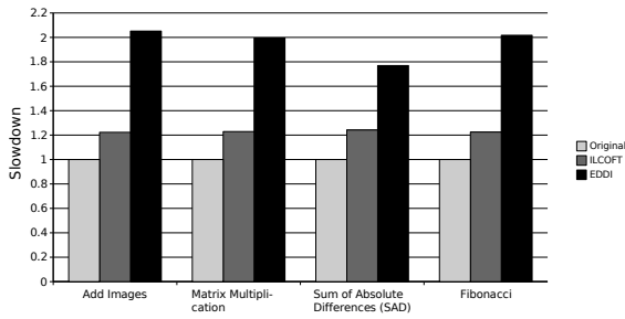
(a) Issue width 1
