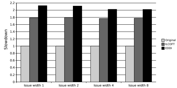
(b) Estimated: JPEG encoder slowdown with protection applied to the whole application. Based on the assumption that for the rest of the application (except the IDCT kernel), EDDI introduces 100% overhead.
