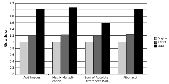
(b) Issue width 2
