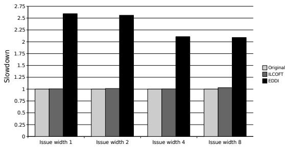
(a) Simulated: IDCT kernel slowdown, accumulated for all its invocations in JPEG encoding.
